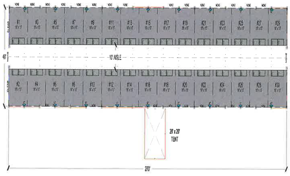
FLOOR PLAN
